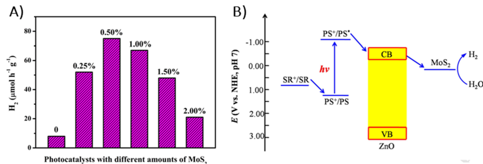
Fig. 40 (A) Photocatalytic \text{H}_2 evolution over ZnTCPP/ \text{MoS}_2 /ZnO photocatalysts with different co-catalyst loadings in a 0.2 M TEOA aqueous solution under visible light irradiation ( \lambda > 420 nm). (B) Suggested mechanism for visible-light-induced hydrogen production using ZnTCPP/ \text{MoS}_2 /ZnO, photosensitizer (PS): ZnTCPP, sacrificial reagent (SR): TEOA. Reproduced with permission from ref. 176. Copyright 2015 Elsevier.
