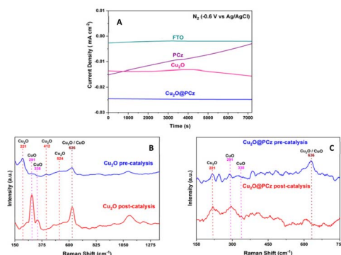
Fig. 9 Stability tests for the \text{Cu}_2\text{O}@PCz electrode and its components on applying a potential of -0.6\text{ V} vs. \text{Ag}/\text{AgCl} in the presence of \text{N}_2 : (A) galvanostatic curves for: FTO (green), PCz (purple), \text{Cu}_2\text{O} (pink), and \text{Cu}_2\text{O}@PCz (blue). (B) Raman spectra of the \text{Cu}_2\text{O} electrode before and after electrocatalysis. (C) Raman spectra of the \text{Cu}_2\text{O}@PCz electrode before and after electrocatalysis.
