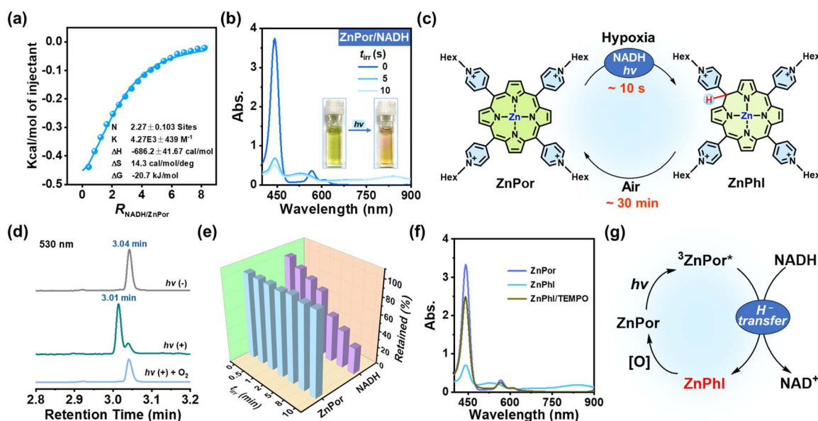
Fig. 3 (a) ITC data measured by titrating 8 mM NADH into 0.2 mM ZnPor in 10% DMSO/PBS. (b) Time-dependent UV-vis spectra of ZnPor (20 μM) and NADH (200 μM) in deoxygenated PBS upon LED light irradiation ( \lambda 405 nm and 25 mW cm -2 ). Inset: photographs of the solution containing ZnPor and NADH in deoxygenated PBS before and after light irradiation. (c) The illustration of the conversion process between ZnPor and ZnPhl. (d) UPLC analysis of the solution containing ZnPor (20 μM) and NADH (200 μM) in deoxygenated pH 7.4 PBS before and after light irradiation ( \lambda 405 nm, 25 mW cm -2 , and t_{\text{irr}} = 5 s), and after exposure to oxygen following irradiation. (e) Time-dependent percentage of remaining ZnPor and NADH in the solution containing ZnPor (20 μM), NADH (200 μM) and TEMPO (10 mM) in deoxygenated PBS upon LED light irradiation ( \lambda 405 nm and 25 mW cm -2 ). (f) UV-vis spectra of solution containing ZnPhl before and after the addition of TEMPO (10 mM). (g) Proposed mechanism of the ZnPor/ZnPhl cycle in the presence of NADH and light.
