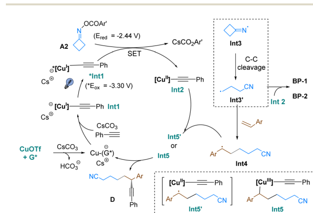
Scheme 5 Proposed catalytic cycle.
