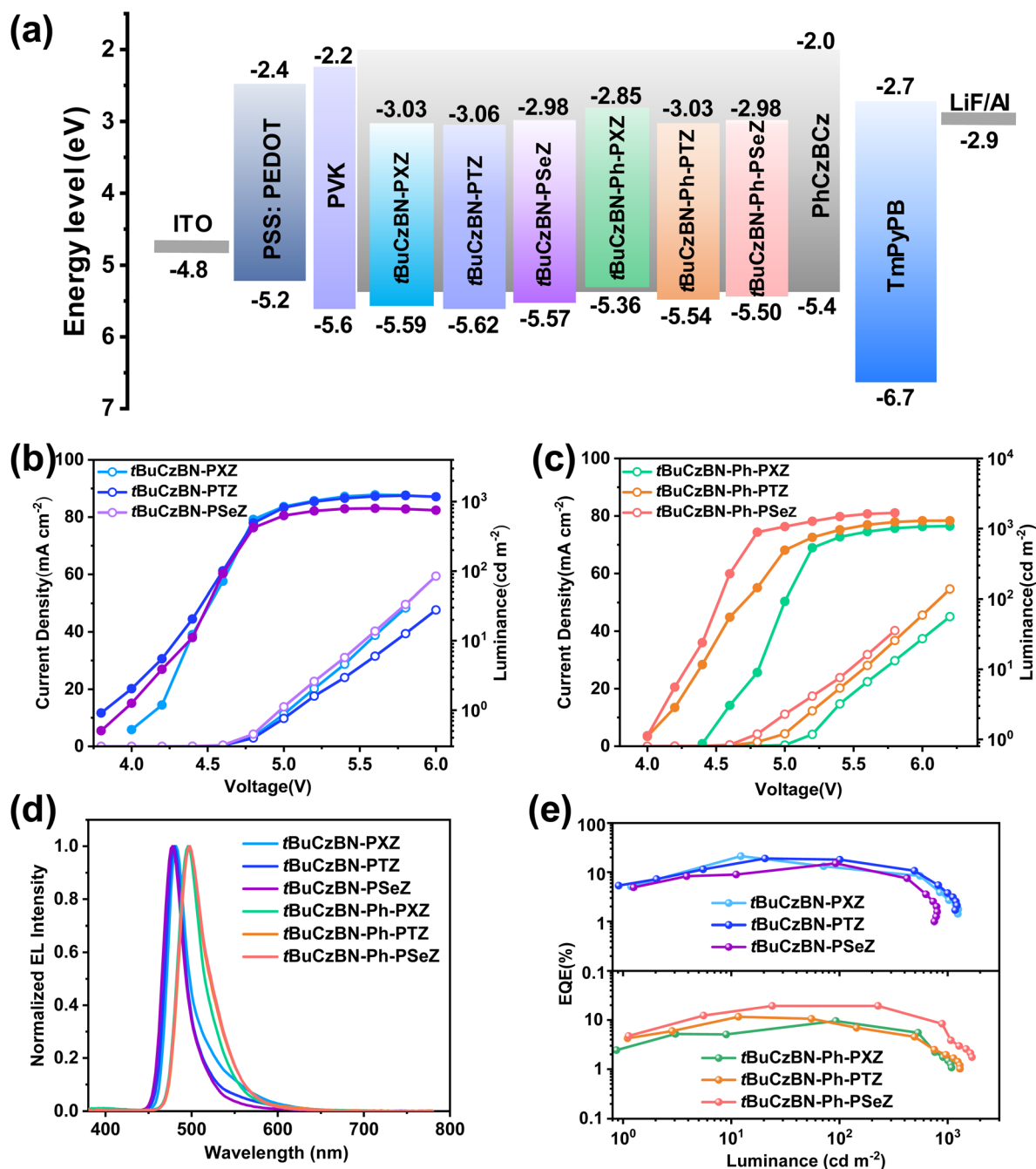
Fig. 6 (a) Device architecture and energy-level diagrams of the functional materials for solution-processed OLEDs. Current density and luminance versus voltage ( J - V - L ) characteristics for (b) tBuCzBN-PXZ, tBuCzBN-PTZ, and tBuCzBN-PSeZ; (c) tBuCzBN-Ph-PXZ, tBuCzBN-Ph-PTZ, and tBuCzBN-Ph-PSeZ. (d) EL spectra recorded at 6 V. (e) External quantum efficiency-luminance (EQE- L ) plots.
