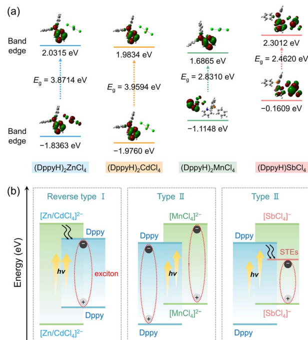
Fig. 4 (a and b) Orbital energy levels and corresponding electronic charge densities for the VBM and CBM as well as band alignments of (DpppyH) n MCl 4 (M = Zn 2+ , Cd 2+ , Mn 2+ , and Sb 3+ ).
