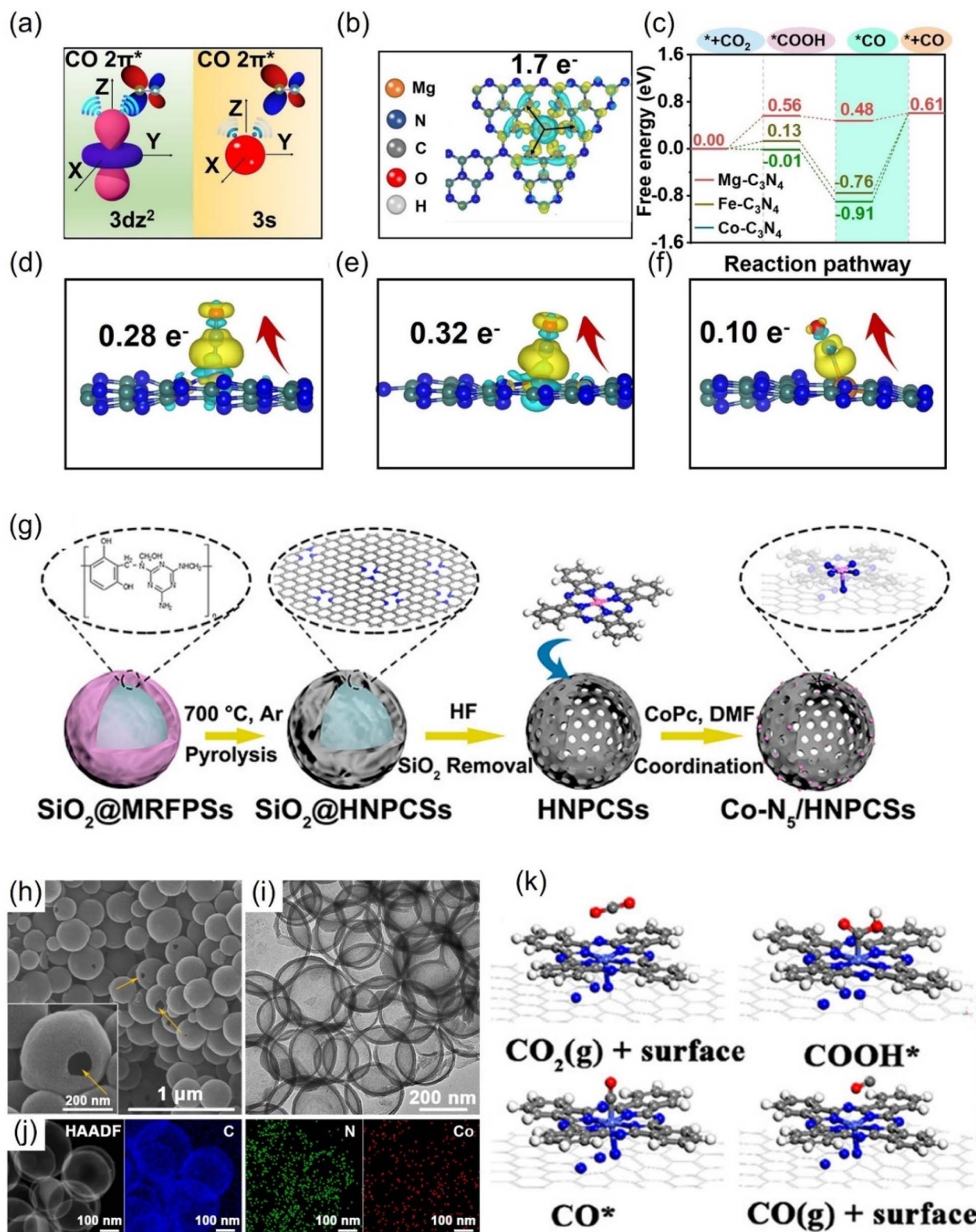
Fig. 17 (a) Comparison of the schematic diagram for CO adsorbed on 3d_{z^2} and 3s orbitals. (b) The charge density differences and Bader charge transfer for Mg- C_3N_4 . (c) Free energy diagram and (d–f) charge density differences and Bader charge transfer for CO adsorbed on Co- C_3N_4 , Fe- C_3N_4 and Mg- C_3N_4 . (g) Schematic illustration, (h) SEM, (i) TEM, (j) HAADF-STEM and EDS images and (k) optimized structures for the intermediates. (a–f) Reproduced with permission. 201 Copyright 2021, Wiley-VCH GmbH. (g–k) Reproduced with permission. 131 Copyright 2018, American Chemical Society.
