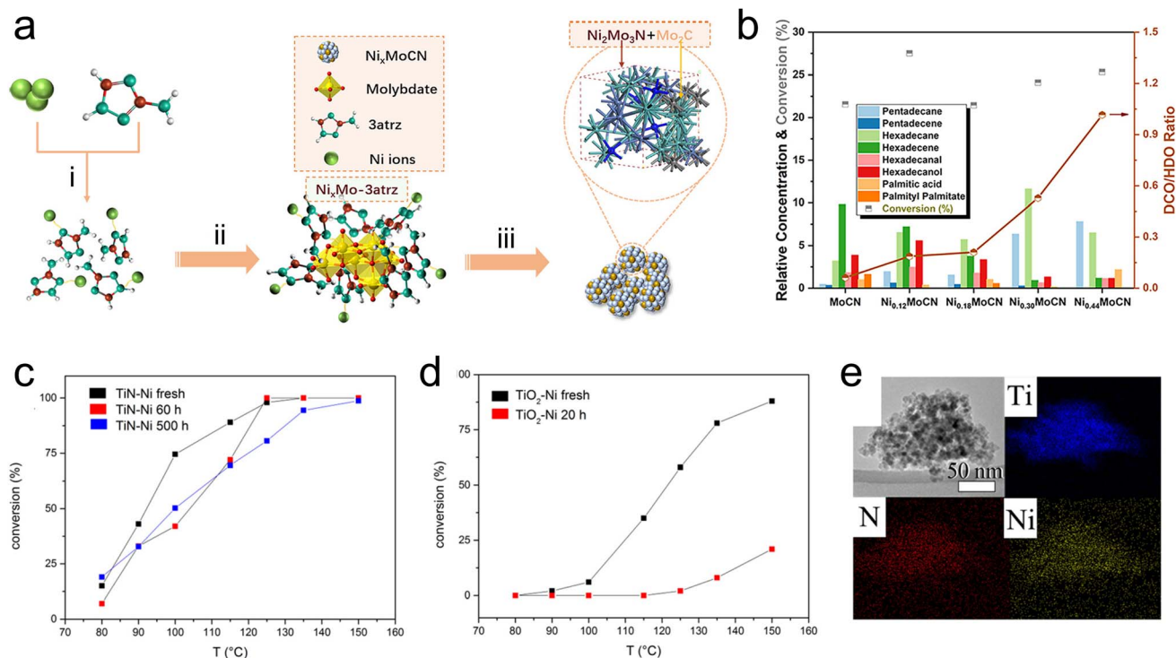
Fig. 6 TMNs for biomass upgrading. (a) Scheme showing synthesis procedure of \text{Ni}_x\text{MoCN} via (a) reaction of Ni nitrate and 3-amino-1,2,4-triazole (3atzr), (ii) addition of Mo to produce organic-inorganic precursor, and (iii) in situ pyrolysis. (b) Product distribution during the reaction of methyl palmitate. (c and d) Conversion of benzyl phenyl ether after continuous reaction of Kraft lignin for 20 h, 60 h, or 500 h. (e) XDS mapping of TiN-Ni catalyst. (a and b) Reprinted from ref. 100 with permission from the American Chemical Society, Copyright 2022. (c–e) Reprinted from ref. 106 with permission from the American Chemical Society, Copyright 2016.
