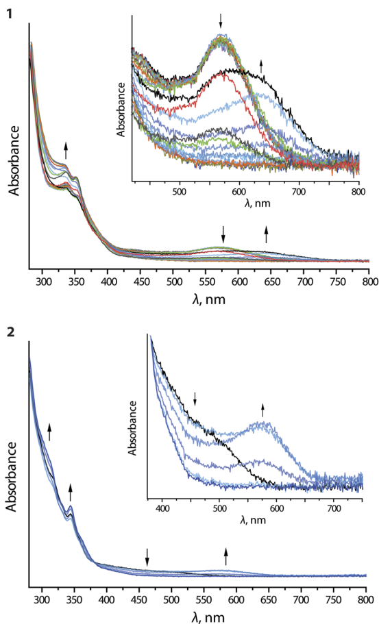
Fig. 8 UV-vis absorption spectra recorded during anodic electrolysis (oxidation) of complexes 1 and 2 in n\text{Bu}_4\text{NPF}_6/\text{DMF} .
