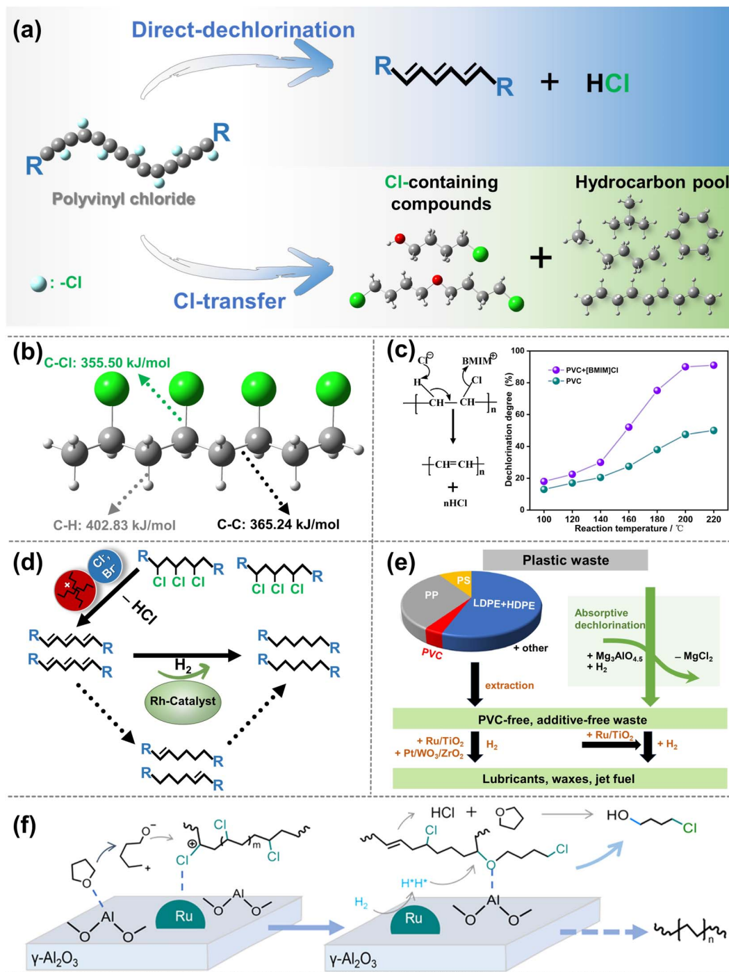
Fig. 7 (a) Schematic diagrams of the upgradation of polyvinyl chloride when C_{aliph}-C_{Cl} bonds are activated over the dual sites. (b) The molecular formula and bond energy of PVC. Reproduced with permission from ref. 127. Copyright 2022 Royal Society of Chemistry. (c) The Schematic picture and the dechlorination effect of [BMIM]Cl on PVC at different temperatures. Reproduced with permission from ref. 134. Copyright 2010 Royal Society of Chemistry. (d) The Schematic picture of the ionic liquid dechlorination/catalytic hydrogenation process. Reproduced with permission from ref. 135. Copyright 2023 Royal Society of Chemistry. (e) Pathways from plastic waste to valuable products. Reproduced with permission from ref. 132 and copyright 2023 Nature. (f) The possible catalytic mechanism of Cl-transfer reaction. Data collected from ref. 141 and copyright 2023 Elsevier.
