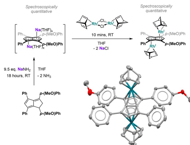
Fig. 8 Top: one-pot-synthesis of anti - [\text{Rh}^{\text{I}}(\text{NBD})]_2[\mu\text{-}\eta^5\text{:}\eta^5(\text{P}^t\text{MeOPh})_2\text{Ph}_2\text{Pn}] ( [\text{Rh}(\text{NBD})]_2[7] ). Bottom: single crystal X-ray structure of [\text{Rh}(\text{NBD})]_2[7] with thermal ellipsoids at the 50% probability level (hydrogen atoms omitted for clarity).
