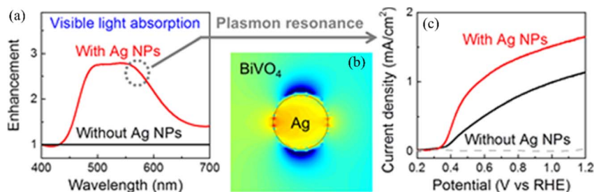
Fig. 8 Applications of plasmon-enhanced photocatalytic water splitting with a Ag NP-impregnated BiVO 4 composite: (a) absorption enhancement of BiVO 4 with and without Ag NPs; (b) simulated light absorption distribution of BiVO 4 with a Ag NP; and (c) current density as a function of the potential of BiVO 4 with and without Ag NPs. 68 Reproduced from ref. 68 with permission from the American Chemical Society, copyright [2018].
