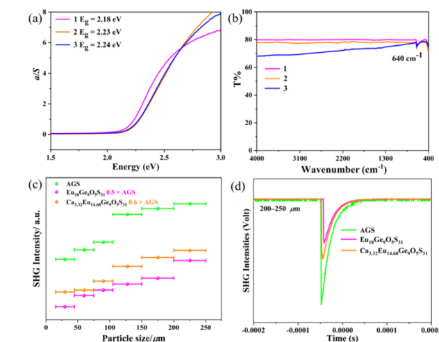
Fig. 2 (a) The UV-vis-NIR diffuse reflection and (b) IR spectra of 1 – 3 ; (c) size-dependent SHG responses and (d) SHG intensities at 200–250 μm of 1 , 2 and AGS under 2.1 μm laser radiation.
