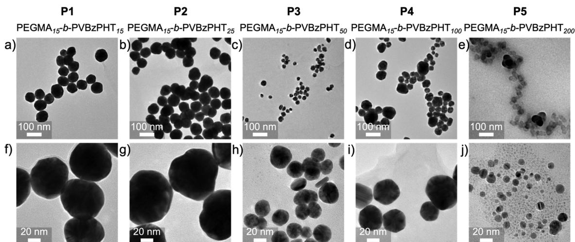
Fig. 5 Representative TEM images for \text{PEGMA}_{15}\text{-}b\text{-PVBzPHT}_n copolymer: P1 (a & f), P2 (b & g), P3 (c & h), P4 (d & i), and P5 (e & j).
