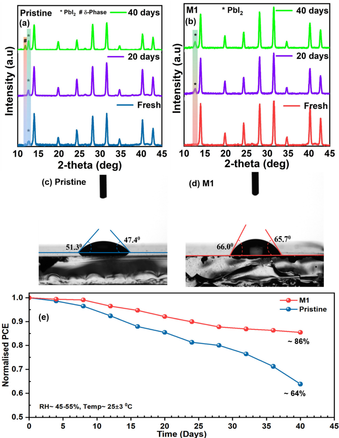
Fig. 7 (a and b) XRD patterns of pristine and optimized perovskite films measured under fresh conditions, after 20 and 40 days by storing under ambient conditions ( RH \approx 45 – 55\% at a temperature of 25 \pm 3 °C), (c and d) contact angles of pristine and optimized perovskite films, and (e) stability testing data of pristine and modified devices stored under ambient conditions ( RH \approx 45 – 55\% at a temperature of 25 \pm 3 °C in the dark).
