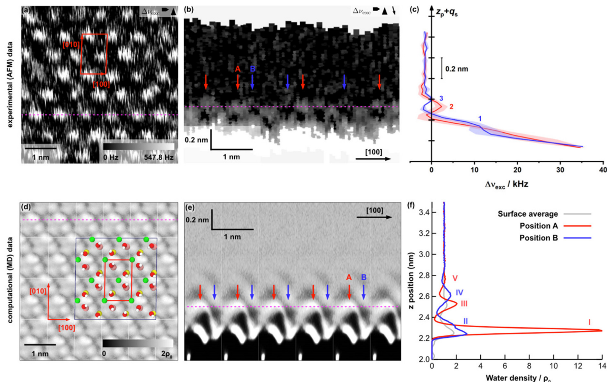
Fig. 4 Results for the (001) microcline–water interface from two- and three-dimensional AFM experiments (a–c) and MD simulations (d–f). (a) Drift-corrected two-dimensional 5 \times 5 nm 2 AFM image. The determined unit cell (shown in red) has dimensions of 0.85 \times 1.31 nm 2 and an angle of 85.7^\circ . (b) Slice normal to the microcline (001) surface extracted from a 3D AFM map taken along the [100] direction. The y position at which the slice normal to the surface where extracted corresponds to the dashed magenta line in the 2D AFM image in (a), which correlates with the lateral slice on peak position 2 (see Fig. S4(b) † ). Two different positions A and B (highlighted by red and blue arrows) can be identified. The dashed magenta line corresponds to the z position where the 2D AFM image in (a) was taken. (c) Averaged \Delta\nu_{\text{exc}} vs. z_p + q_s profiles taken at the red and blue positions in (b). Three peaks labelled (1)–(3) can be identified. (d) Water density map parallel to the (001) microcline–water interface within the second hydration layer between z = 2.50 and 2.55 nm from MD simulations. The positions of K + ions and hydroxyl groups in the bulk-terminated surface are overlaid and the surface unit cell is shown in red. The dark blue marked box displays the original simulation box with a size of 2 \times 3 unit cells in [010] and [100] directions. (e) Vertical slice through the water density extracted along the [100]-direction at the y position indicated by the dashed magenta line in panel (d). The dashed magenta line indicates the z position of the horizontal slice shown in panel (d). As in the 3D AFM data, two different positions A and B can be identified, marked by red and blue arrows. (f) Water density profiles extracted at the two positions A and B, averaged over an area of 0.1 \times 0.1 nm 2 in each of the six surface unit cells. Additionally, the average water density profile over the entire surface (grey) is shown. Five peaks can be identified in total, labelled (I)–(V). The reference bulk water density is \rho_0 = 33.7 nm −3 .
