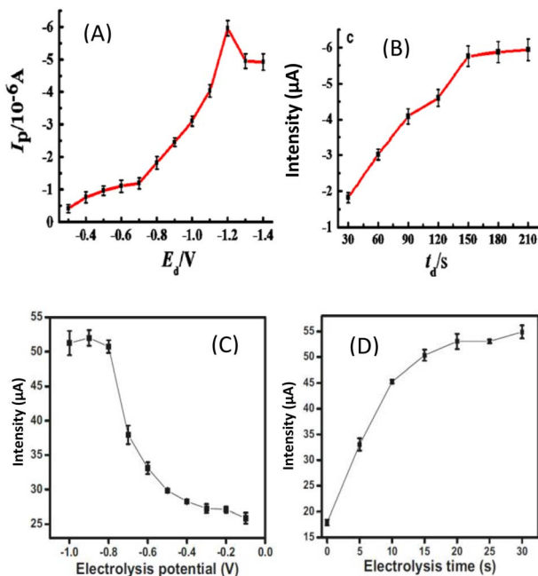
Fig. 9 Electrolysis potential (A) and electrolysis time (B) in 10 \mu\text{M} \text{Pb}^{2+} in 0.1 M acetate buffer (pH 5.4) recorded at a \beta -CD-rGO/GCE. This figure has been reproduced from ref. 51 with permission from Springer, copyright 2016. Electrolysis potential (C) and electrolysis time (D) in 2 \mu\text{M} \text{Pb}^{2+} in 0.1 M acetate buffer (pH 5) recorded at a GCE/NHAPPO.5-CA- \beta -CD. This figure has been reproduced from ref. 40 with permission from Springer-Verlag GmbH Germany., copyright 2021.
