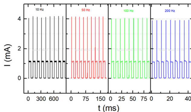
Fig. 9 I-t curves for the Ag@40 device at different chopper frequencies and at a fixed power density of 317 mW cm -2 .
