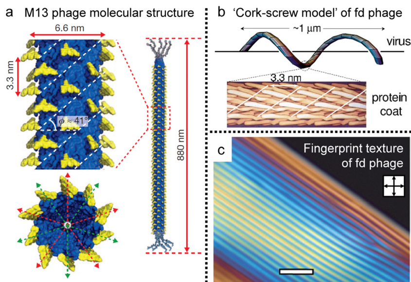
Fig. 12 Filamentous bacteriophages and their anisotropy. (a) Molecular structure of the M13 bacteriophage. (b) Schematic illustration of 'cork-screw model' of fd virus. (c) Cholesteric phase of concentrated viral solution exhibiting fingerprint texture under POM. (a) Reproduced from ref. 120 with permission from Springer Nature, copyright 2011. (b) Reproduced from ref. 115 with permission from American Physical Society, copyright 2003. (c) Reproduced from ref. 117 with permission from Royal Society of Chemistry, copyright 2009.
