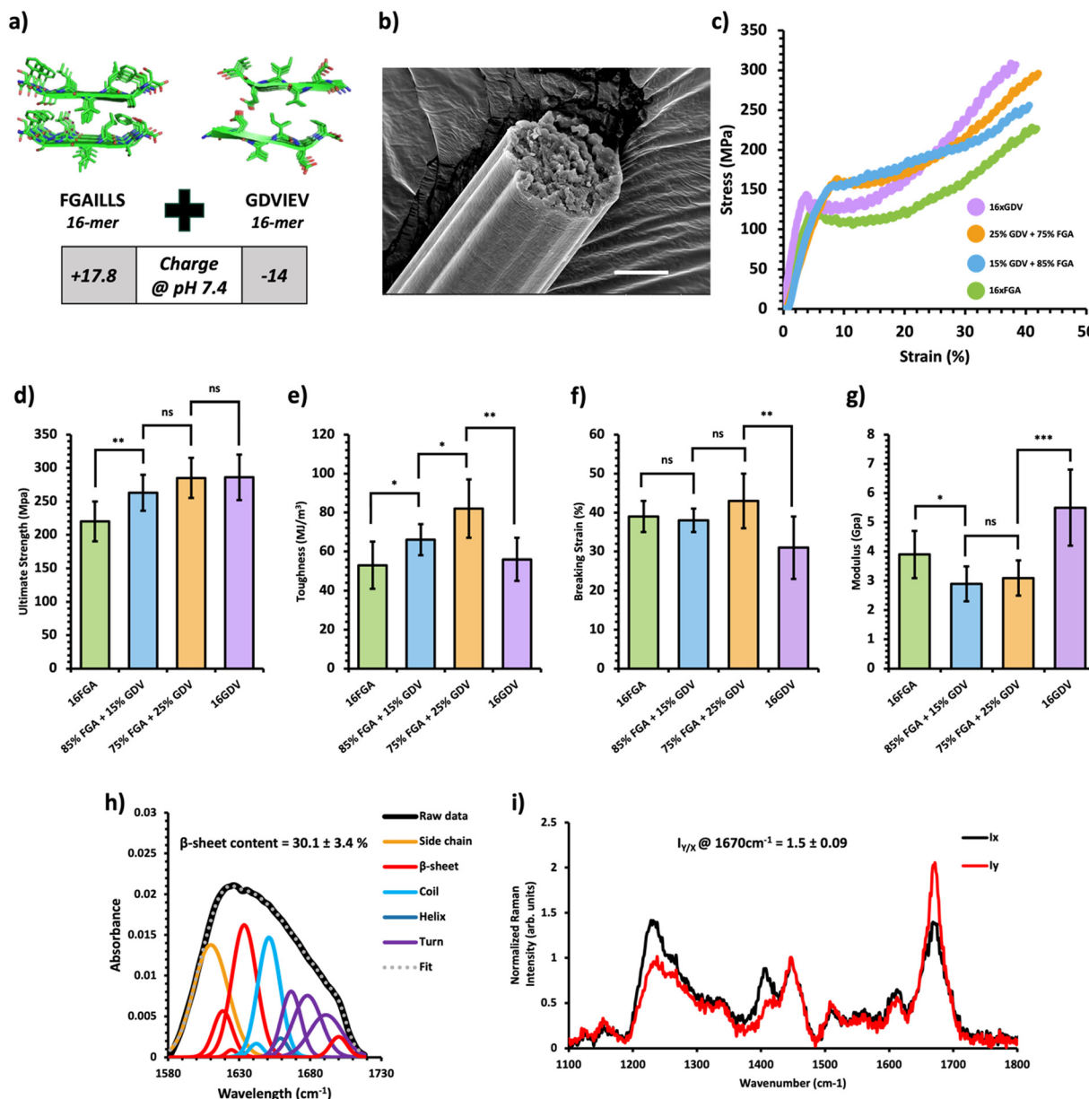
Fig. 3 Mechanical and structural properties of protein charge-based composite fibers. (a) Crystal structure of the FGAILLS (PDB: 5E61) and GDVIEV (PDB: 3SGS) amyloid peptides. Polymerized amyloid-silk proteins containing 16 repeats of the FGAILLS peptide (+17.8 charged at pH 7.4) or 16 repeats of the GDVIEV peptide (−14 charged at pH 7.4) were mixed to generate protein charge-based composite fibers. (b) Representative S.E.M. image of the 75:25 16xFGA/16xGDV protein composite fibers. Stretched fiber pieces were imaged after tensile testing. Scale bars represent 10 \mu\text{m} . (c) Representative stress-strain curves from tensile testing of the protein charge-based composite fibers at different mixture ratios. (d)–(g) Ultimate tensile stress (d), toughness (e), breaking strain (f), and Young's modulus (g) of the protein charge-based composite fibers. Error bars represent standard deviation. ^{ns}P > 0.05 , ^{*}0.01 < P < 0.05 , ^{**}0.001 < P < 0.01 , ^{***}0.0001 < P < 0.001 , ^{****}P < 0.0001 , two-tailed unpaired t test. (h) FTIR analysis of post-spin drawn 75:25 16xFGA/16xGDV protein composite fibers. The amide I band was deconvoluted into 11 Gaussian peaks and the average \beta -sheet content was determined using steps outlined in the 'Methods' section. (i) Raman spectra of stretched 75:25 FGA/GDV protein composite fibers oriented perpendicular ( I_{\perp} ; red line) or parallel ( I_{\parallel} ; blue line) to the direction of the incident laser polarization. Spectra shown were acquired by averaging spectra from three separate fibers. Orientation sensitivity was determined by calculating the average peak intensity ratio at 1670\text{ cm}^{-1} ( I_{\parallel}/I_{\perp} ).
