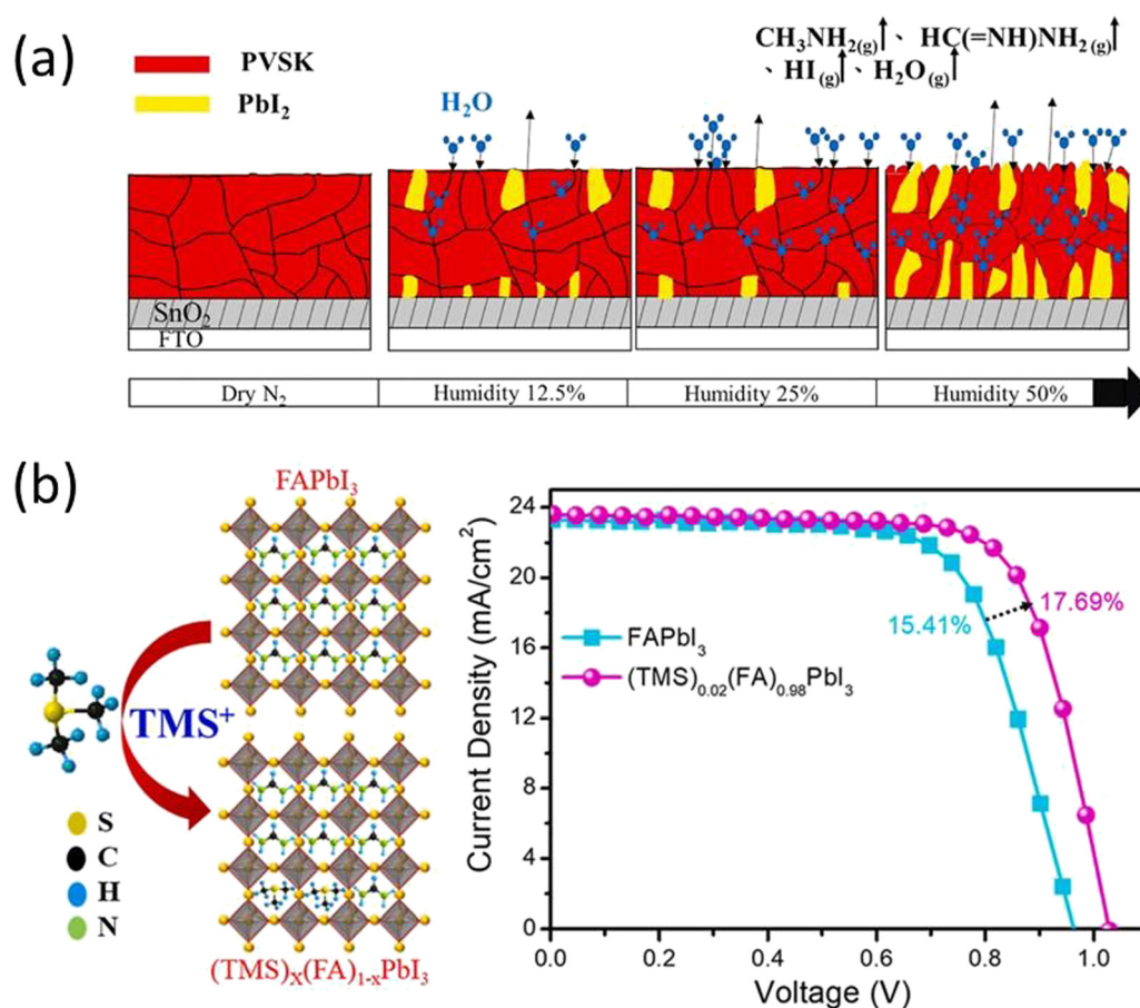
Fig. 2 (a) Water molecules in contact with (\text{Cs}_{0.05}\text{FA}_{0.85}\text{MA}_{0.15}\text{Pb}(\text{I}_{0.85}\text{Br}_{0.15})_3) perovskite crystal grain boundaries form a hydrated phase; \text{PVSK} in the figure. Continuous heating during the annealing process returns partially hydrated phases to the original perovskite phase, while a portion of the samples underwent degradation to form \text{CsI} , \text{CH}_3\text{NH}_2 , \text{HC(=NH)NH}_2 , \text{HI} , \text{PbI}_2 , \text{PbBr}_2 , and \text{H}_2\text{O} . Increasing the humidity levels to 50% accelerated degradation, resulting in the formation of large quantities of \text{CH}_3\text{NH}_2 , \text{HC(=NH)NH}_2 , and \text{PbI}_2 . Reproduced from ref. 69 with permission from John Wiley and Sons, copyright 2022. (b) Schematic crystal structure and JV plots of \text{FAPbI}_3 before and after \text{TMS}^+ incorporation. Reproduced from ref. 73 with permission from Elsevier, copyright 2022.
