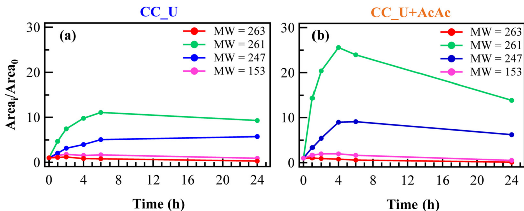
Fig. 6 Evolution of FNT degradation products during electro-Fenton experiments, using CC_U (a) and CC_U + AcAc (b) as working electrodes. For all species, the Area i /Area 0 ratio was calculated as the ratio between the chromatographic peak areas at the i -th time and at time = 0 h.
