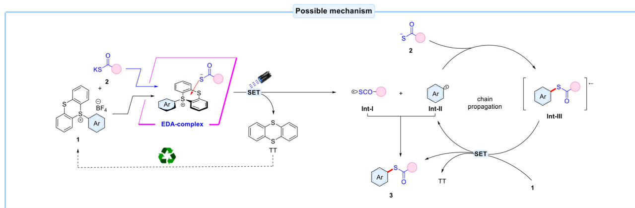
Scheme 3 Possible mechanism.
