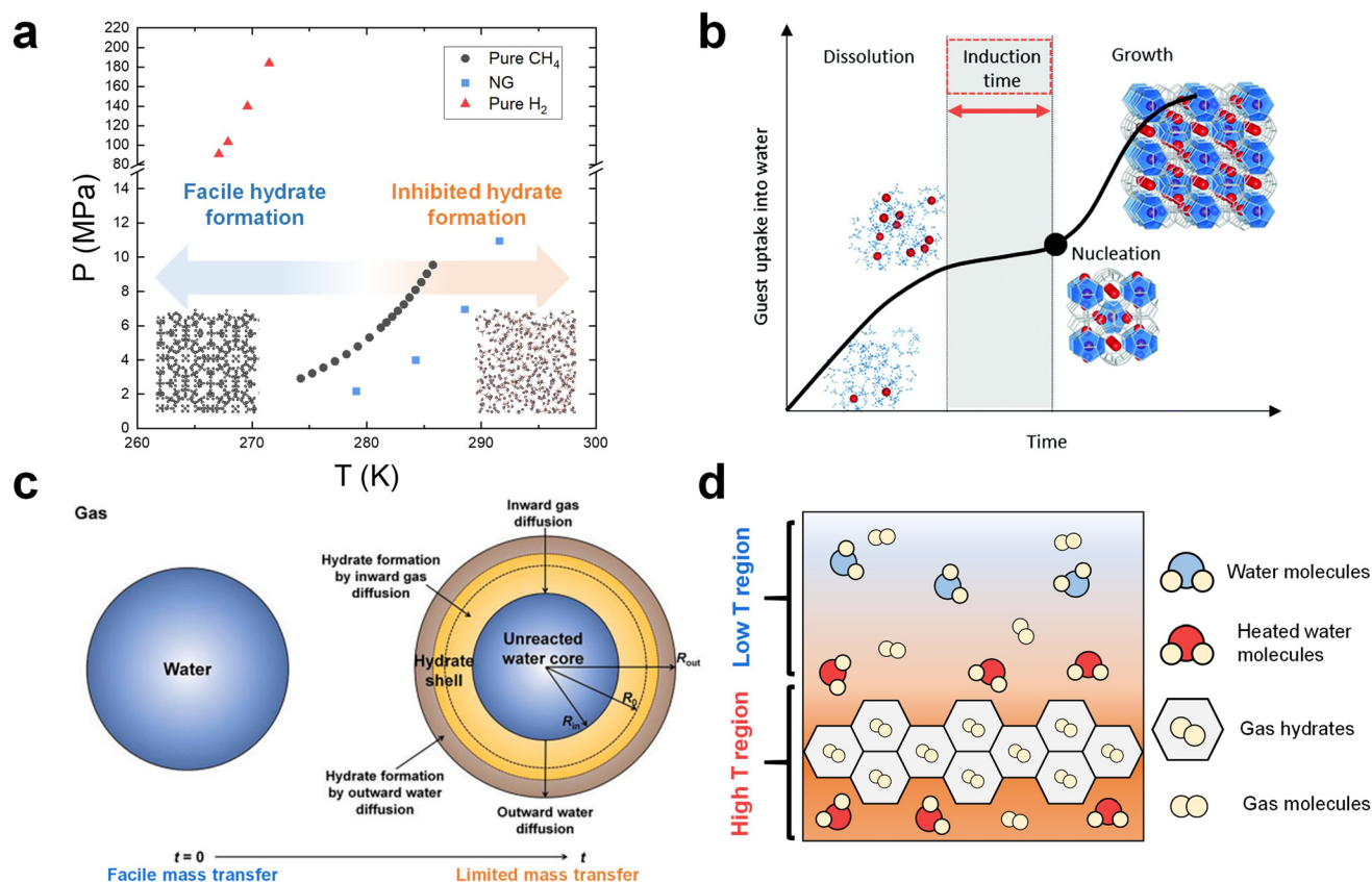
Fig. 1 (a) Phase equilibrium boundaries of CH 4 , 116 NG, 115 and H 2 117 hydrates. (b) General time dependence of the hydrate crystallization process. Reproduced with permission. 122 Copyright 2020, Royal Society of Chemistry. (c) Schematic illustration of hydrate formation on a water droplet in the diffusion-controlled regime. Reproduced with permission. 143 Copyright 2023 Elsevier. (d) Schematic of heat boundaries in the system where growing hydrates exist.
