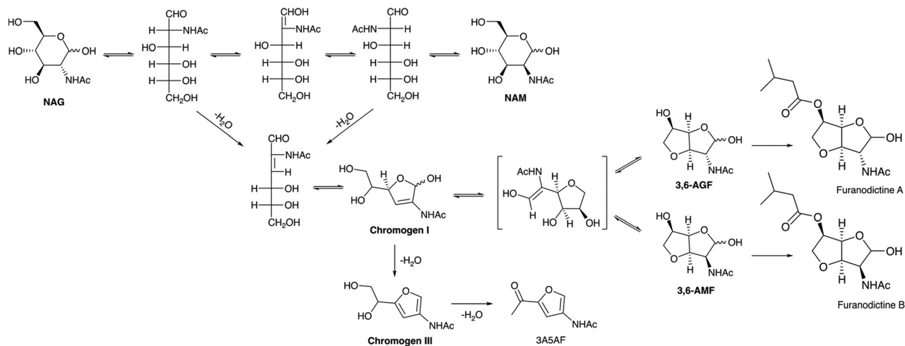
Scheme 4 Probable reaction pathway for the formation of Chromogen I, Chromogen III, 3A5AF and 3,6-anhyrohexofuranoses from NAG.
