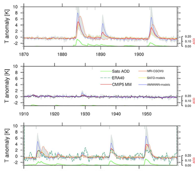
Fig. 5 Stratospheric warming at 50 hPa between 30 °S and 30 °N in the lower stratospheric region after nine major volcanic eruptions in the period between 1870 and 2000 from both historical observations and modeling simulations. Reprinted with permission of the publisher from Driscoll et al. , J. Geophys. Res. Atmos. , 2012, 117 , 17105.
