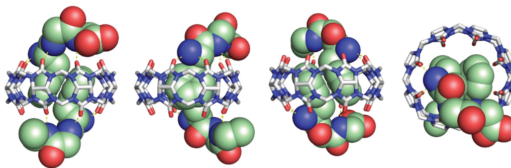
Fig. 8 Rendering of the crystal structure of the \text{Q8} \cdot (\text{H-Phe-Gly-Gly-OH})_2 complex shown from different viewing angles. The peptide is shown as space-filling, and Q8 as sticks. Peptide carbons are green. Q8 carbons are grey. Oxygens are red. Nitrogens are blue. Hydrogens are not shown. Yellow dashes show key intermolecular electrostatic interactions. 18
