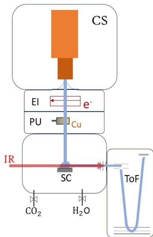
Figure 1. Schematic sketch of the ClusTOF experiment, more details can be found in the text. HNDs are produced by the cluster source (CS). After multiply charging the droplets via electron impact (EI), they are doped with evaporated copper in the pick-up chamber (PU), followed by the pick-up of CO 2 and, if desired, H 2 O. After cluster formation, the HNDs collide with a surface (SC), liberating He-tagged dopants feasible for analysis and detection with the time-of-flight (ToF) mass spectrometer. Action spectroscopy is achieved by irradiating the extracted cluster ions with an IR laser before entering the ToF.
