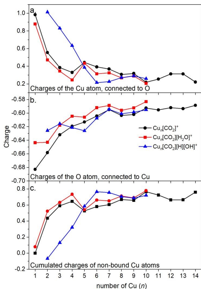
Figure 6: a. Charges of the Cu atom which is connected to the \text{CO}_2 in \text{Cu}_n[\text{CO}_2]^+ . b. Charges of the O atom in \text{Cu}_n[\text{CO}_2]^+ which is connected to the cluster. c. Cumulated charges of the copper atoms except the Cu atom which is connected to the \text{CO}_2 in \text{Cu}_n[\text{CO}_2]^+ (copper atoms not bound to \text{CO}_2 ).
