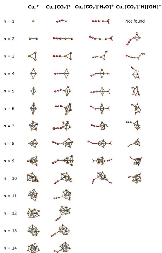
Figure 3: Lowest energy isomers for \text{Cu}_n^+ , \text{Cu}_n[\text{CO}_2]^+ , \text{Cu}_n[\text{CO}_2][\text{H}_2\text{O}]^+ , and \text{Cu}_n[\text{CO}_2][\text{H}][\text{OH}]^+ in the studied binding modes.
