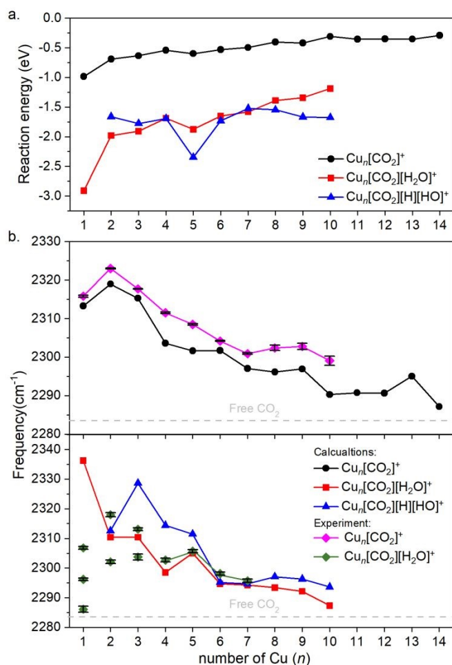
Figure 4: a. Binding energies of the cluster adducts depicted on Figure 3. b. Top: Frequencies of the asymmetric stretching vibrational mode of the bound \text{CO}_2 on corresponding adducts are depicted. Bottom: The frequency of the same vibration, when water is co-adsorbed. The diamonds denote the experimental results, which include error bars. Note that the error bars are often smaller than the symbols; therefore, a black color is used to represent them. Additionally, for \text{Cu}_n[\text{CO}_2][\text{H}_2\text{O}]^+ , for n = 1-3 the symbols are not connected, since it is not clear which of them might originate from the \nu_3 vibration. The dashed grey line represents the vibration of free \text{CO}_2 .
