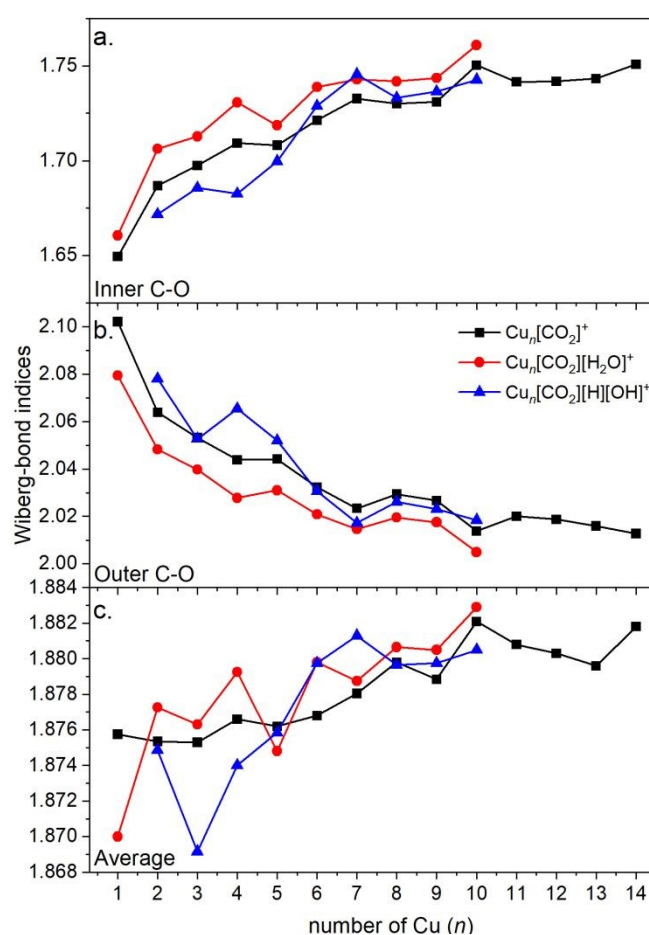
Figure 7: Wiberg bond indices of a. the C-O bond (where oxygen is connected to the cluster, i.e. inner oxygen); b. the C-O bond (where oxygen is not connected to the cluster, i.e. outer oxygen); c. both C-O bonds (inner and outer) with respect to the cluster size.
