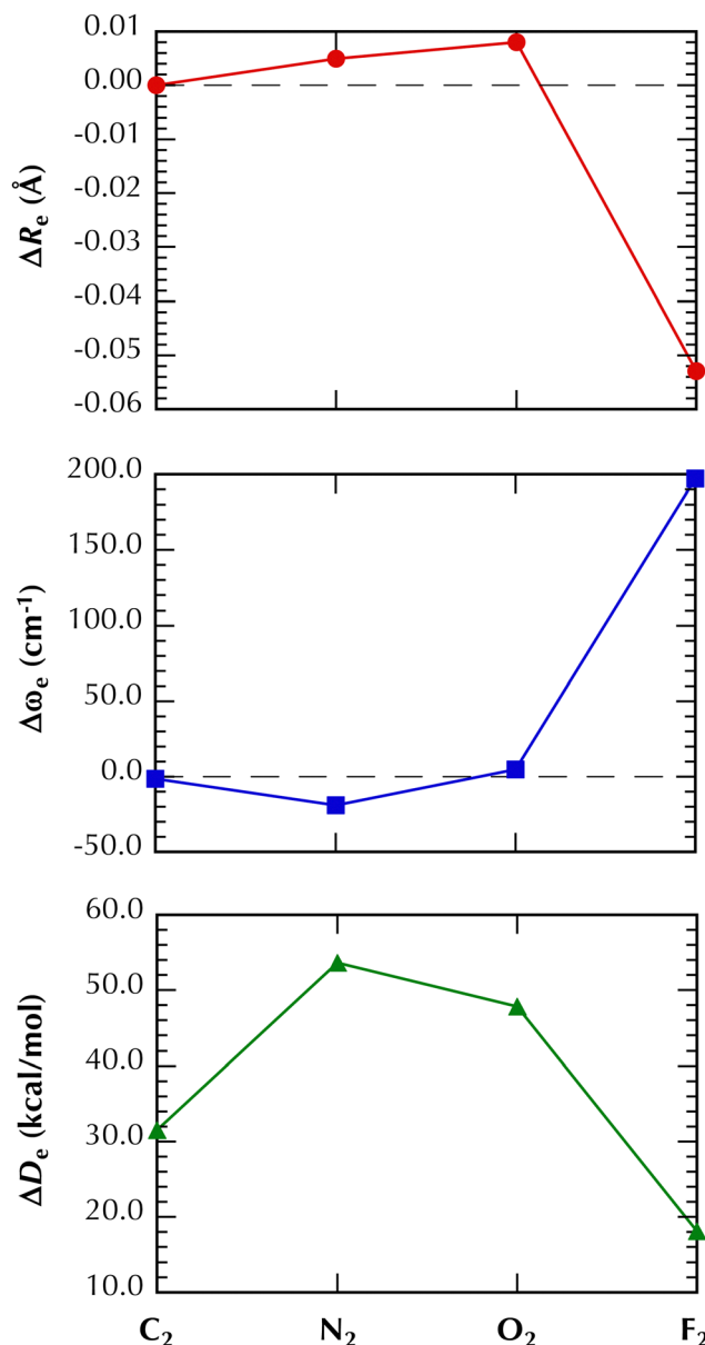
Fig. 1 Changes in the spectroscopic constants of C_2 - F_2 resulting from inclusion of dynamical electron correlation, e.g., \Delta R_e = R_e(\text{vCAsCI}) - R_e(\text{SCGVb}) .
