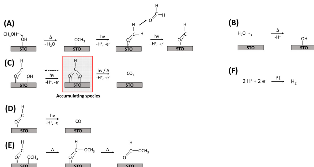
Fig. 6 Proposed reaction mechanism for the thermal-assisted photocatalytic methanol oxidation in the gas phase (steps A)–(F) including the main carbon-based reactants, intermediates, and products as well as the reduction of H + at Pt NPs. The accumulated formate species was highlighted (see (C)) as it is proposed to be the main deactivating species. Note that, the regeneration of hydroxyl and methoxy groups must be considered to fulfil the hydrogen balance. Step F does not take into account the total amount of H + produced by other steps. The trace compounds CH 4 , dimethoxy methane and dimethyl ether were omitted.
