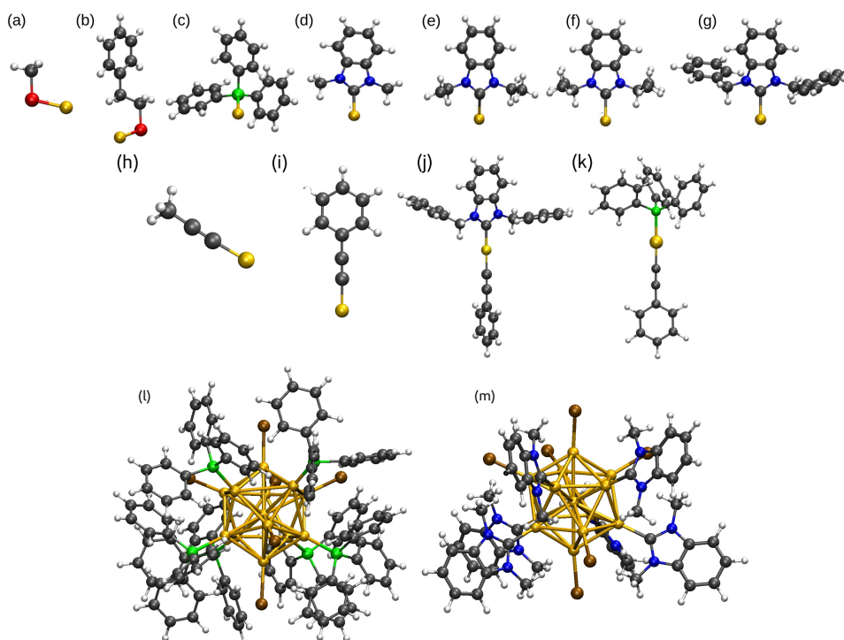
Fig. 1 Molecular structures of PBE optimized M-L complexes (a-i), L 1 -M-L 2 (j and k), and two PPh 3 and NHC Me protected metal clusters (l and m, respectively). (a) Au-SCH 3 , (b) Au-SC 8 H 9 , (c) Au-PPh 3 , (d) Au-NHC Me , (e) Au-NHC Et , (f) Au-NHC iPr , (g) Au-NHC Bn , (h) Au-CCMe, (i) Au-CCPh, (j) NHC Bn -Au-CCPh 3 , (k) PPh 3 -Au-CCPh, (l) [Au 13 (PPh 3 ) 6 Br 6 ] - , (m) [Au 13 (NHC Me ) 6 Br 6 ] - . Au, yellow; S, red; C, black; H, white; P, green; N, blue; Br, brown. The optimized structures of Au-L, L 1 -Au-L 2 , and [Au 13 L 6 Br 6 ] - are representative of all M-L and L 1 -M-L 2 complexes and ligand protected metal clusters; the atom radius is not precise.
