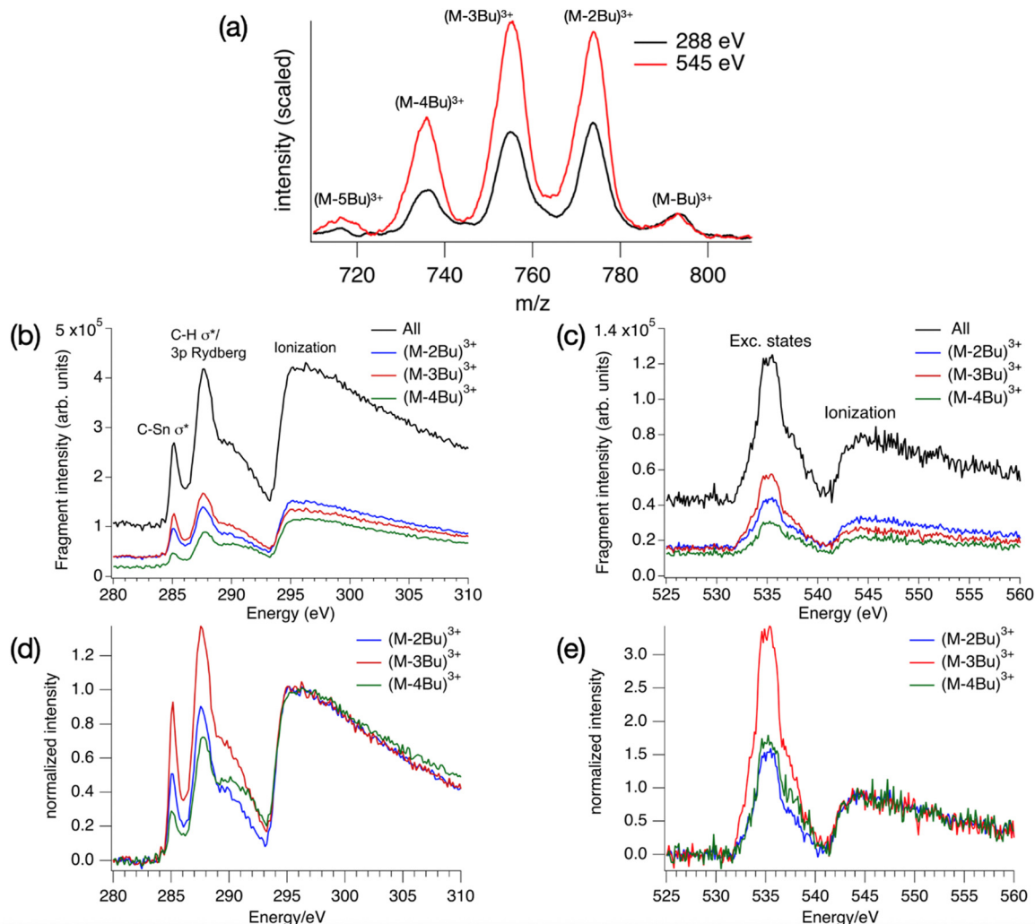
Fig. 6 (a) Photofragmentation mass spectra 288 eV and 545 eV irradiation, scaled to the same intensity of (M-Bu)^{3+} peak, corresponding to the triply charged molecular ion having lost one butyl group. (b) and (c) NEXAMS spectra, obtained by measuring the partial ion yields of the three largest peaks in the mass spectrum as a function of photon energy, corrected for background. (b) Carbon K-edge. (c) Oxygen K-edge. The colored traces give the separate partial ion yields for trications that lost 2, 3 and 4 Bu groups ( (M-2Bu)^{3+} , (M-3Bu)^{3+} , (M-4Bu)^{3+} ). (d) and (e) NEXAMS spectra for the individual ions, scaled to the same intensity at the ionization edge.
