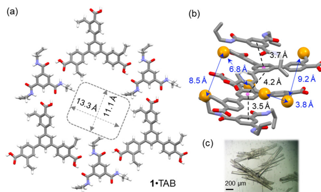
Fig. 1 (a) Single-crystal structure of the 1 ·TAB co-crystal viewed along the b/c plane. (b) The ABBA-type alternative packing of 1 and TAB, viewed along the a -axis. The π-π stacking distances and distances between the terminal carbon atoms of the styrene moieties are highlighted. (c) An image of 1 ·TAB co-crystals.
