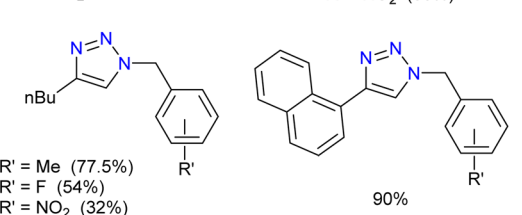
Scheme 39 Substrate scope of CuAAC reaction.
