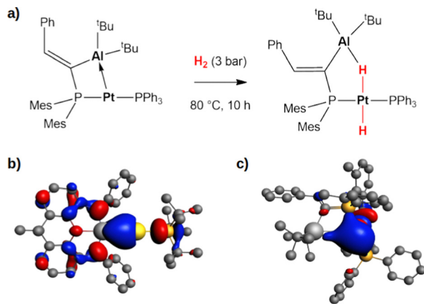
Fig. 5 (a) Experimentally reported reactivity of a Pt \rightarrow Al complex with H_2 . 52 (b) and (c) Isosurfaces of the HOMO of the gold–aluminylyl complex (b) and platinum–aluminum complex (c). The isovalue is 3 m_e a_0^{-3} . The isosurfaces have been taken and adapted with permission from ref. 50 Copyright 2023, Royal Society of Chemistry.
