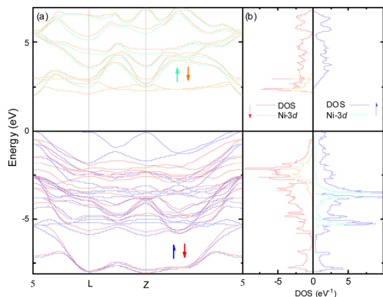
Fig. 2 Calculated electronic structure of NiGa 2 S 4 . (a) Band structure along principal directions of the first Brillouin zone. (b) Density of states (DOS) for the spin-up (↑) and spin-down (↓) channels including PDOS for Ni-3d states.
