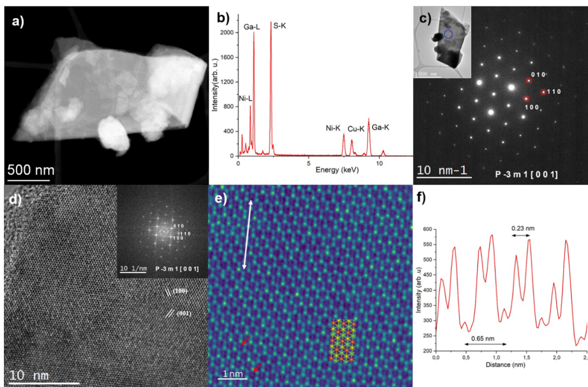
Fig. 3 (a) Low magnification STEM-HAADF image of a NiGa 2 S 4 flake. (b) Corresponding EDS spectrum. (c) SAED pattern acquired on the same flake successfully indexed as corresponding to the NiGa 2 S 4 P\bar{3}m1 crystal structure seen along the [0 0 1] (= [0 0 0 1]) zone axis. The inset displays the corresponding low-magnification TEM image, and the blue circle highlights the area used to acquire the SAED pattern. (d) HR-TEM image acquired on a thin area of the same flake. The inset shows the corresponding FFT pattern. It has been successfully indexed as belonging to the NiGa 2 S 4 P\bar{3}m1 crystal structure seen along the [0 0 1] (= [0 0 0 1]) zone axis. (e) Filtered HR-TEM image corresponding to an enlarged view of Fig. 3d. It is superposed with the NiGa 2 S 4 atomic structure as seen along the [0 0 1] zone axis (Ni: orange, Ga: green, S: yellow). The red arrows highlight the presence of Ni atoms, and the white arrow highlights the area used to extract the intensity profile shown in (b). (f) Intensity profile extracted from the HR-TEM image (white arrow, Fig. 3e).
