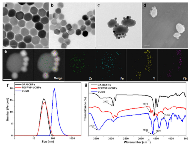
Fig. 1 TEM images of (a) UCNPs ( \text{NaYF}_4: 25\% \text{Yb}^{3+}, 0.9\% \text{Tm}^{3+}, 0.6\% \text{Nd}^{3+} ), (b) dual-ligand PEI/PVP modified UCNPs, and (c) UCMs. (d) SEM images of UCMs. (e) Dark-field TEM images and the corresponding area-elemental mapping of UCMs, including Zr, Fe, Y and Yb. (f) The statistical data showing the size distributions of OA-UCNPs, PEI/PVP-UCNPs and UCMs. (g) FT-IR spectra for OA-UCNPs, PEI/PVP-UCNPs and UCMs. The scale bars indicate 50 nm in all the tested cases.
