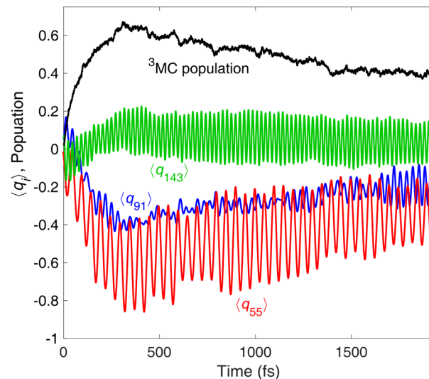
Fig. 7 Average trajectories \langle q_{55} \rangle (red, pyridine ring deformation), \langle q_{91} \rangle (blue, pyridine ring deformation), and \langle q_{143} \rangle (green, internal ligand bending/wagging) of [Fe(bmip) 2 ] 2+ corresponding to three selected ligand modes, as obtained from the simulation with 400 nm excitation. Also shown are the population dynamics of the 3 MC state (black).
