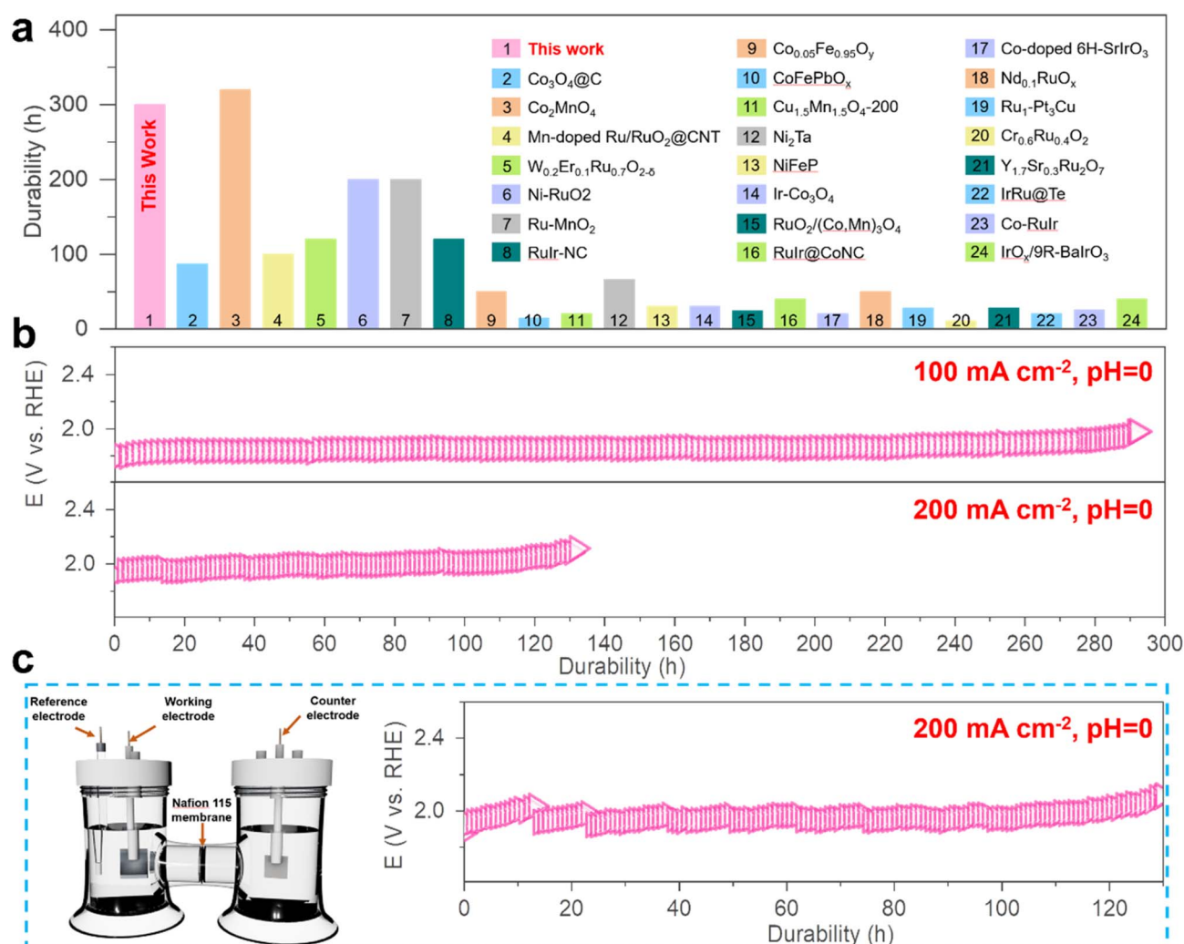
Fig. 3 Stability of MnCoO_x . (a) Comparison of the durability of Mn_1Co_5O_x catalysts in acidic solution with that of other reported catalysts. Of note, samples 1–5 were measured at 100 mA\ cm^{-2} , and the others, at 10 mA\ cm^{-2} . (b) Potential required to reach 100 and 200 mA\ cm^{-2} in 0.5 M H_2SO_4 for Mn_1Co_5O_x measured using chronopotentiometry method. (c) Chronopotentiometric measurement of the Mn_1Co_5O_x catalyst at a constant OER current density of 200 mA\ cm^{-2} recorded in an H-type water electrolysis cell in 0.5 M H_2SO_4 with the anode and cathode separated by a Nafion 115 membrane at room temperature.
