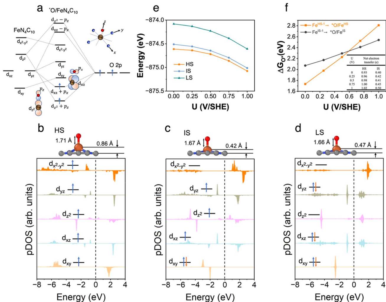
Fig. 4 ^*O/FeN_4C_{10} . (a) Schematics of orbital hybridizations of Fe 3d orbitals in a square-planar ligand field with the 2p orbitals in the O adsorbate. (b)–(d) Atomic structures and pDOS plots of the HS, IS, and LS states of ^*O/FeN_4C_{10} . (e) Spin- and potential-dependent energies of ^*O/FeN_4C_{10} under constant-potential conditions. (f) Spin and potential-dependent ^*O adsorption energies. The inset table shows the net electron transfer in the adsorption process.
