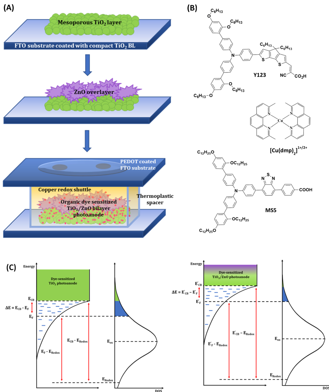
Fig. 1 (A) Fabrication scheme and device architecture of DSCs employing bilayer TiO 2 /ZnO photoanodes. (B) Chemical structure of the organic sensitizers (Y123 and MS5) and the redox mediator ([Cu(dmp) 2 ] 1+/2+ ). (C) Alignment of energy levels of the semiconductor layer and electrolyte. A negative shift in the conduction band edge ( E_{CB} ) of TiO 2 /ZnO electrodes results in reduced overlapping between the oxidized energy states of the electrolyte with the conduction band states (shaded in green) and the gap states (shaded in blue).
