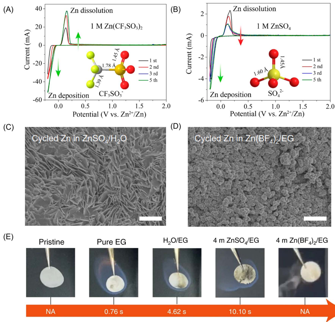
Fig. 6 Cyclic voltammery of the Zn electrode in aqueous electrolyte of (A) 1 M Zn(CF 3 SO 3 ) 2 and (B) 1 M ZnSO 4 at the scan rate of 0.5 mV s -1 between -0.2 and 2.0 V. Reproduced with permission. 102 Copyright 2016, American Chemical Society. Top-view SEM images of the cycled Zn after 20 cycles in (C) the reference aqueous ZnSO 4 electrolyte and (D) the 4 m Zn(BF 4 ) 2 /EG electrolyte. (E) Ignition tests of a pristine glass fibre separator, one saturated with pure EG, a H 2 O/EG solution, a 4 m ZnSO 4 /EG solution and a 4 m Zn(BF 4 ) 2 /EG solution. NA (not applicable) indicates non-flammability. Reproduced with permission. 101 Copyright 2021, Springer Nature.
