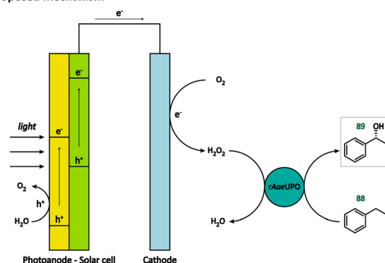
Fig. 14 Cathode-mediated in situ \text{H}_2\text{O}_2 generation for asymmetric C–H oxygenation.
