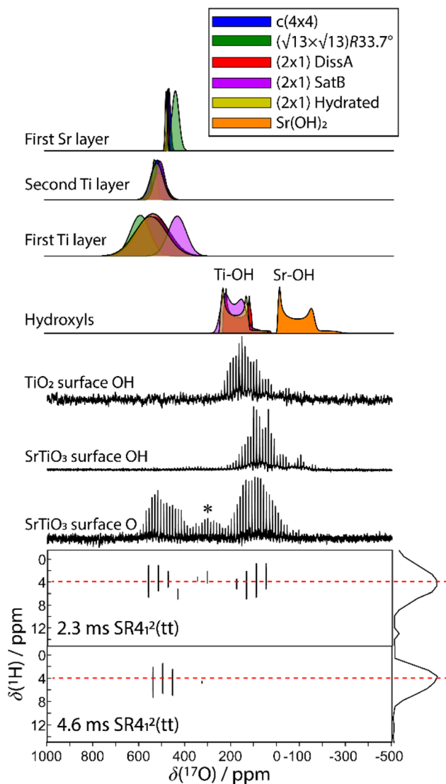
Fig. 5 Experimental (black) D-RINEPT-SR 412 (tt) (bottom) 1D and 2D ^{17}\text{O}\{^1\text{H}\} spectra and ^{17}\text{O}\{^1\text{H}\} PRESTO spectra acquired on STO and anatase titania. Simulated spectra are shown on the top corresponding to the parameters calculated using plane-wave DFT for various surface terminations, as indicated on the figure. An asterisk is used to mark the position of a spinning sideband.
