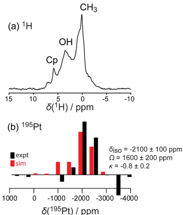
Fig. 6 Simulated (red) and experimental (black) ^1\text{H} MAS (a) and ^{195}\text{Pt} perfect-echo RESPOR (b) solid-state NMR spectra acquired on a MeCpPtMe 3 /STO material.
