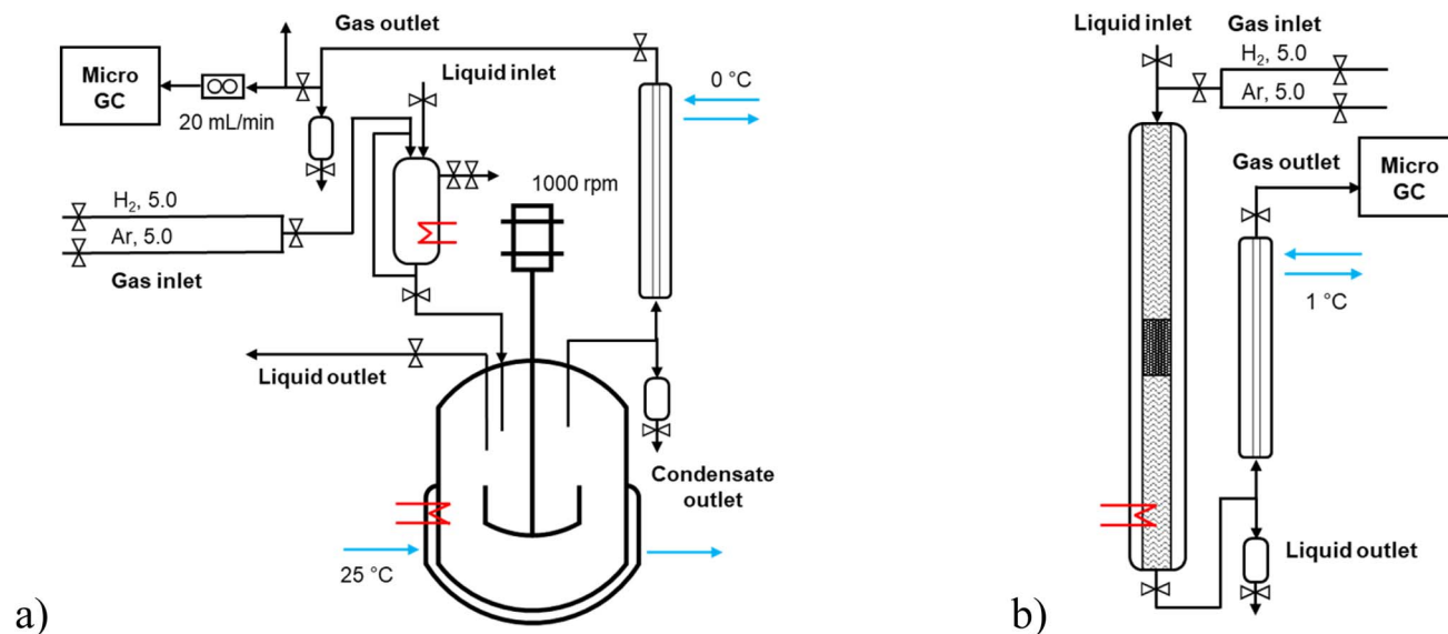
Fig. 1 The scheme of the experimental setup: (a) batch and (b) continuous modes.
