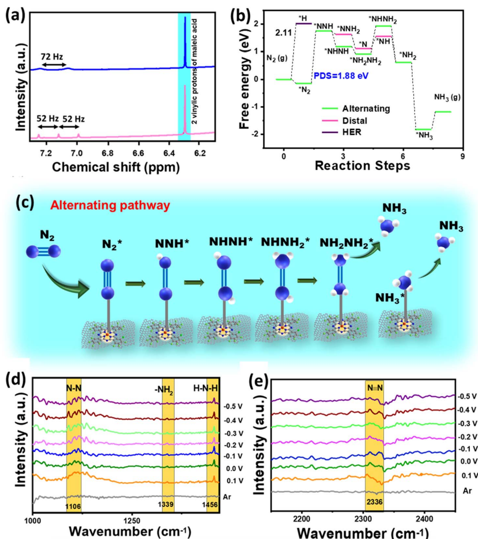
Fig. 6 (a) Isotope labeling experiment displaying ^1\text{H-NMR} spectra obtained after the NRR in 1 M \text{Na}_2\text{SO}_4 with ^{14}\text{N}_2 (pink) and ^{15}\text{N}_2 (blue) as feed gases, (b) Free energy profile of the NRR for F-CuPc-G, (c) scheme showing the reaction mechanism of F-CuPc-G during NRR follows alternating pathway. (d and e) In situ ATR-FTIR spectra obtained for F-CuPc-G.
