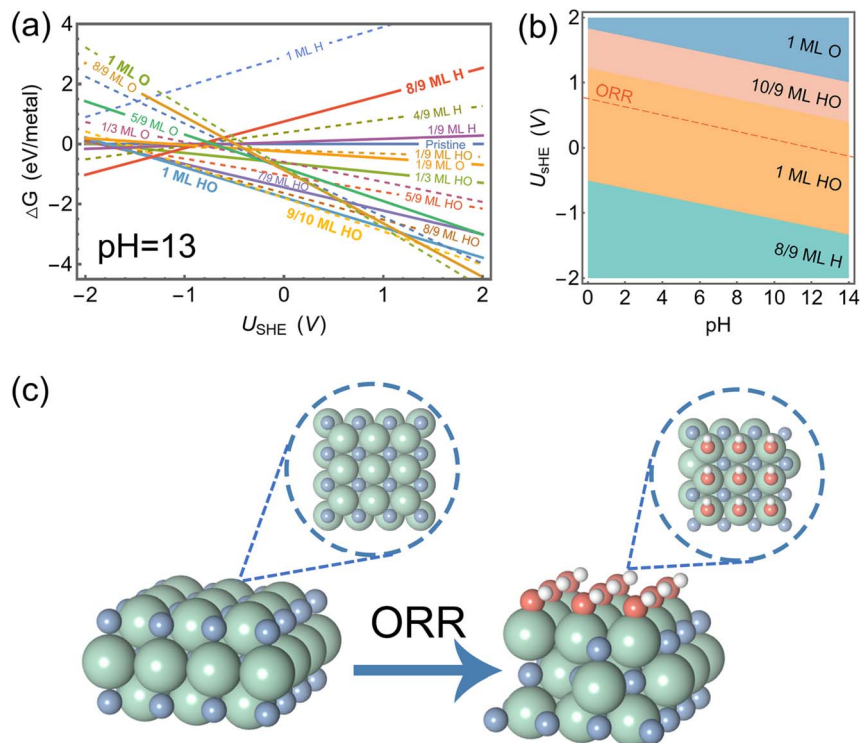
Fig. 1 (a) Calculated 1D surface Pourbaix diagram as a function of potential (vs. SHE) (pH = 13; T = 298.15 K). (b) 2D surface Pourbaix diagram as a function of potential (vs. SHE) and pH ( T = 298.15 K). (c) Optimized structures of the ZrN(100) surface before and after HO^* coverage under ORR conditions. Insets are the corresponding top views. Green, blue, red, and white spheres denote Zr, N, O, and H, respectively.
