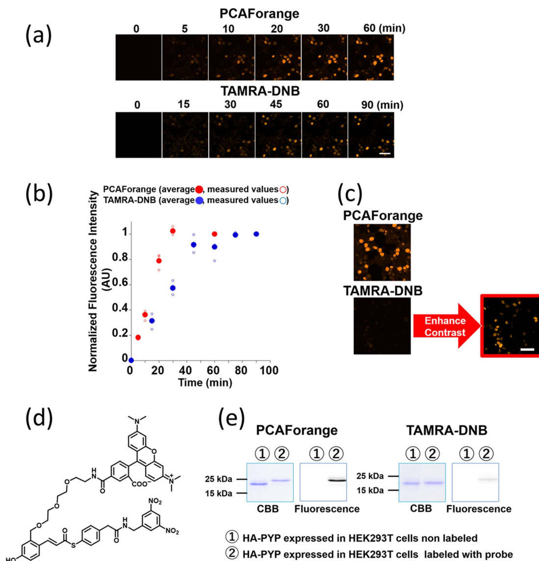
Fig. 4 Comparison of the labeling performance of PCAForange against TAMRA-DNB. (a) Time-lapse imaging of PYP-NLS expressed in HEK293T cells labeled with 1 \mu\text{M} PCAForange or 1 \mu\text{M} TAMRA-DNB. Scale bar: 50 \mu\text{m} . (b) Quantification of the fluorescence intensity of PYP-NLS labeled with PCAForange (red solid circles) and TAMRA-DNB (blue solid circles). Data points plotted are means of the mean of triplicate measurements (open circles) with error bars representing the standard deviations. (c) Comparison of the brightness of PCAForange- and TAMRA-DNB-labeled PYP-NLS in HEK293T cells imaged at the same laser intensity. Due to low signal intensity, TAMRA-DNB-labeled cells could only be visualized with contrast enhancement. Scale bar: 50 \mu\text{m} . (d) Chemical structure of TAMRA-DNB. (e) SDS-PAGE analysis of labeling efficiency of PCAForange and TAMRA-DNB in live HEK293T cells.
