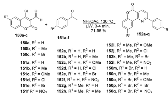
Scheme 54 Synthesis of diverse pyrido[3,2-c]coumarins 152a–q .
