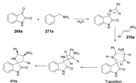
Scheme 96 Plausible mechanism for the synthesis of representative molecule 272a.
