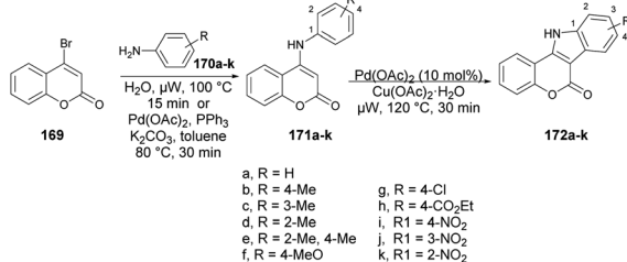
Scheme 61 Synthesis of azacoumestans 172a–k.
