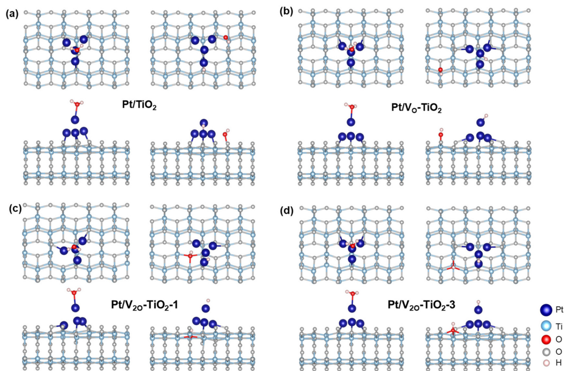
Fig. 6 Structures for \ast\text{H}_2\text{O} and \ast\text{OH}/\ast\text{H} adsorbed on the (a) \text{Pt}/\text{TiO}_2 , (b) \text{Pt}/\text{V}_2\text{O}_5\text{-TiO}_2 , (c) \text{Pt}/\text{V}_2\text{O}_5\text{-TiO}_2\text{-1} , (d) \text{Pt}/\text{V}_2\text{O}_5\text{-TiO}_2\text{-3} surfaces.
